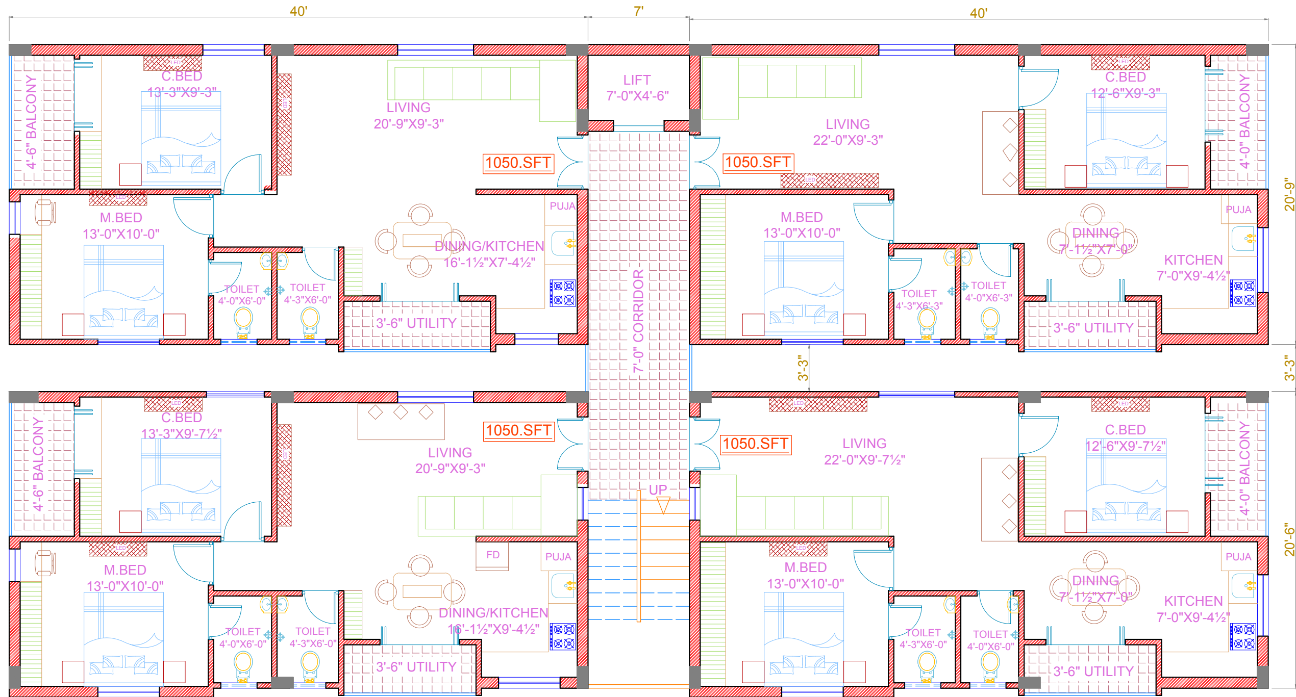
TYPICAL FLOOR PLAN 5UPPER FLOORS
